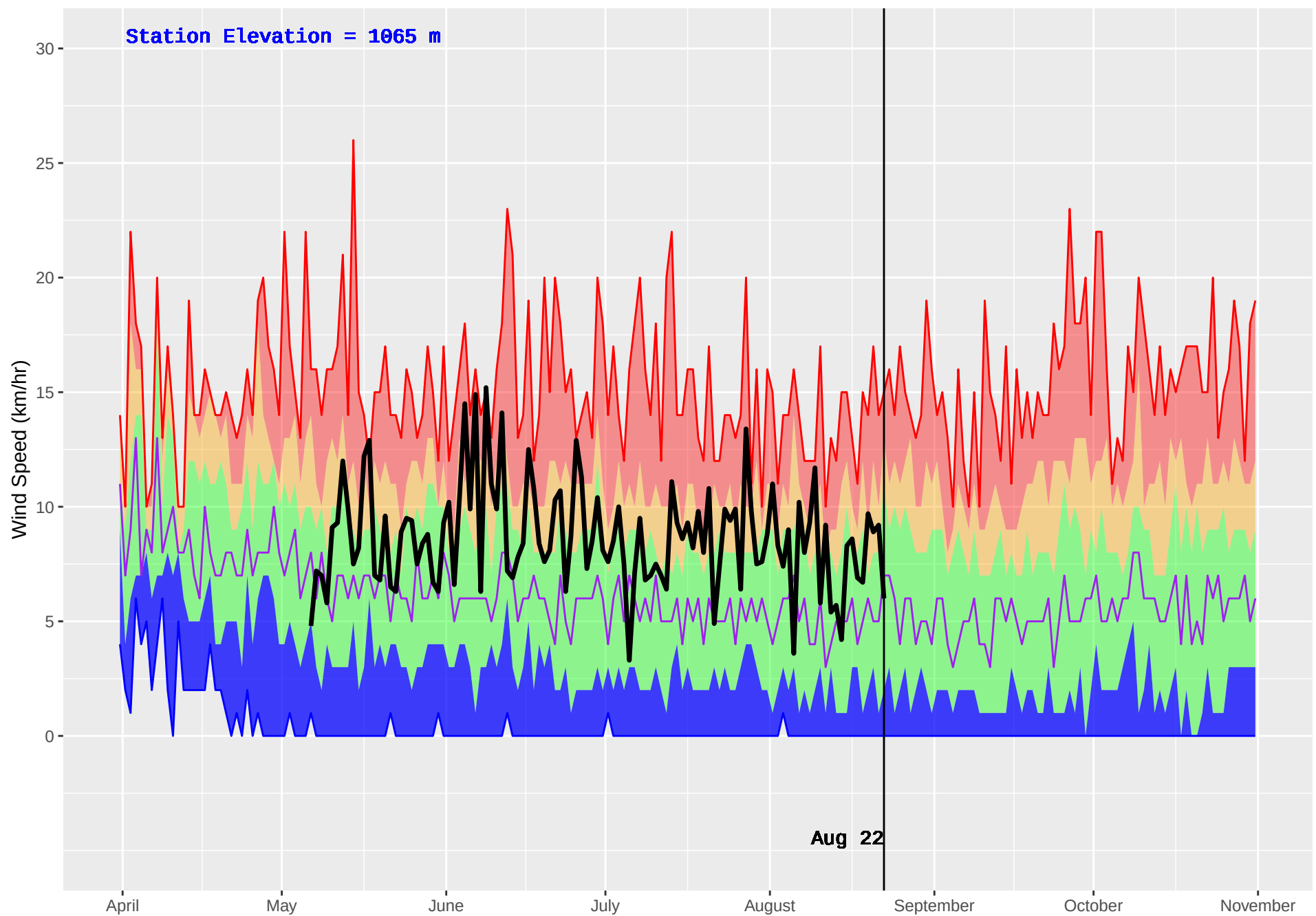
PLACE LAKE (212) : Historical (1981–2016) and Current (2018) Daily Wind Speed
