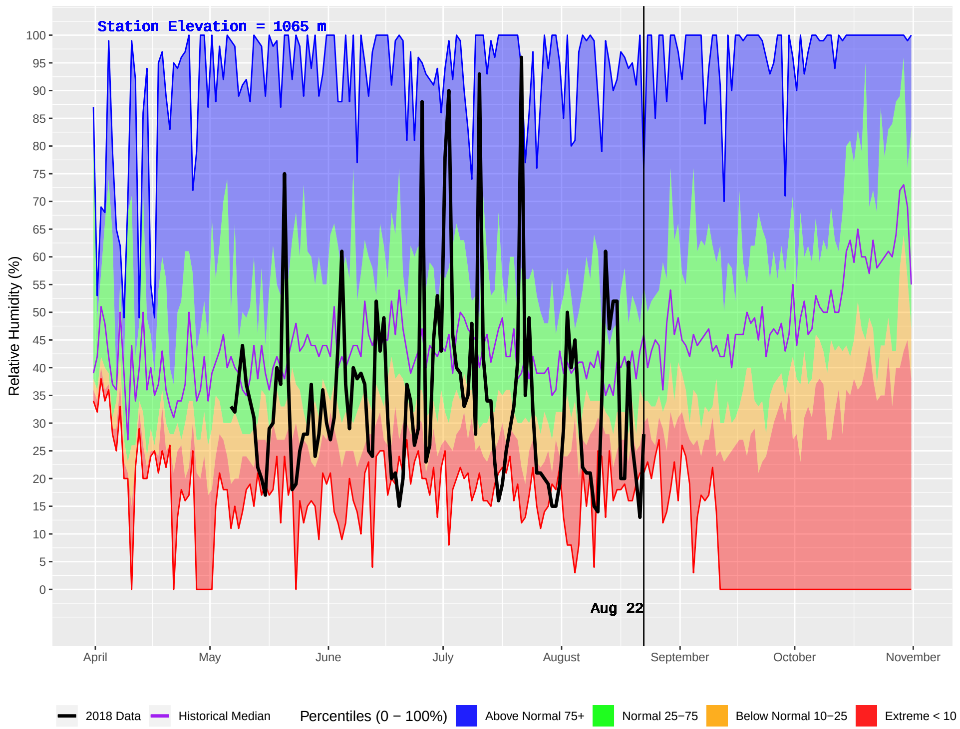
PLACE LAKE (212) : Historical (1981–2016) and Current (2018) Daily Relative Humidity
